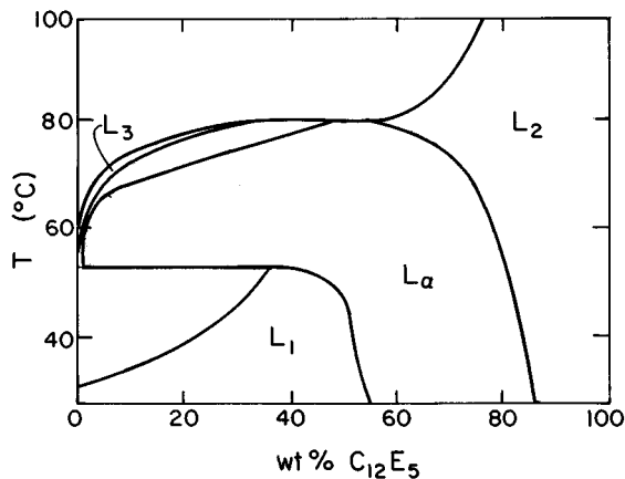
FIG. 1. Phase diagram of water C_{12}E_5 system. The lamellar phase is denoted L_a , while isotropic disordered phases are denoted L_1 , L_2 , and L_3 . The L_1 phase is a micellar fluid; L_3 is the sponge phase. Regions without labels are of two-phase coexistence (after Ref. [1]).
