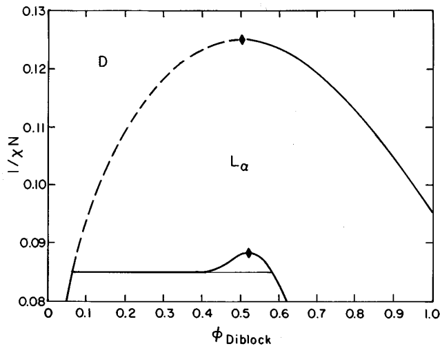
FIG. 2. Phase diagram of the AB -copolymer, A -homopolymer system. The possible occurrence of a hexagonally perforated lamellar phase is ignored. The line of complete unbinding is shown dashed and ends at a Lifshitz point, marked with a diamond. Beyond it is a line of second-order transitions from the disordered phase D to the lamellar phase L_\alpha . The coexistence region between two lamellar phases ends at a critical point, also denoted by a diamond. Regions without labels are of two-phase coexistence.
